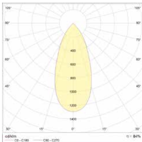
Flood Beam
