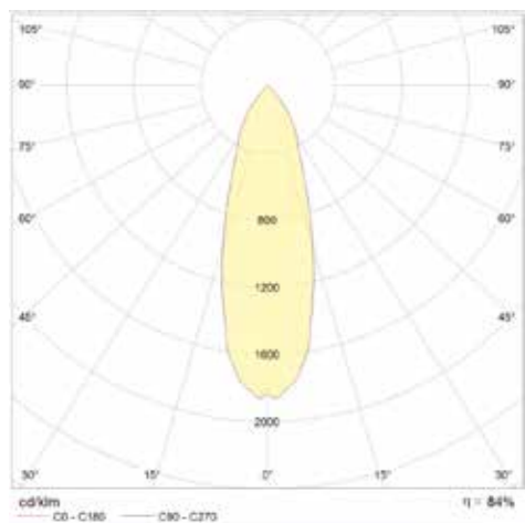
Medium Beam
