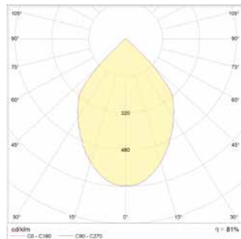
Wide Beam
