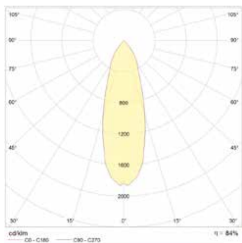
Medium Beam
