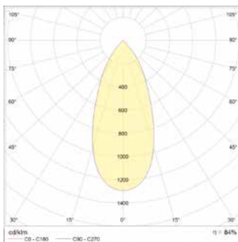
Flood Beam
