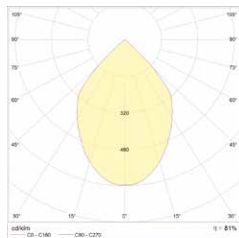
Wide Beam
